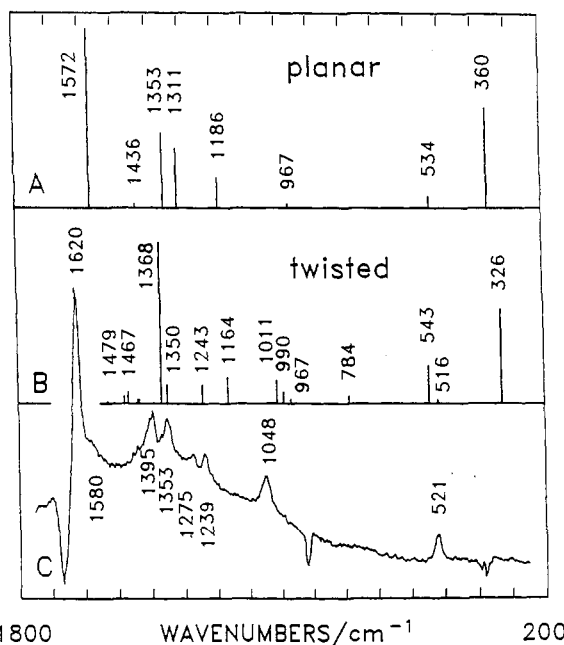
Figure 4. Calculated T_1 state frequencies and resonance Raman intensities of the totally symmetric modes of planar and twisted forms of TMB together with its observed T_1 resonance Raman spectrum. 89 The intensities are taken proportional to the \gamma -values of the T_1 \rightarrow T_n transition ( n = 4 and 5 for planar and twisted forms, respectively).
