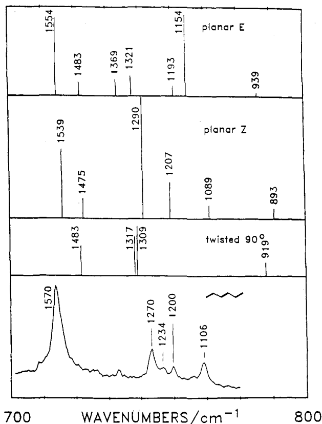
Figure 2. Calculated T 1 state frequencies and resonance Raman intensities of the totally symmetric modes of trans ( E ), cis ( Z ), and twisted forms of hexatriene together with its observed T 1 resonance Raman spectrum. 89 The intensities are taken proportional to the γ-values of the T 1 → T n transition (n = 5 and 6 for planar and twisted forms, respectively).
